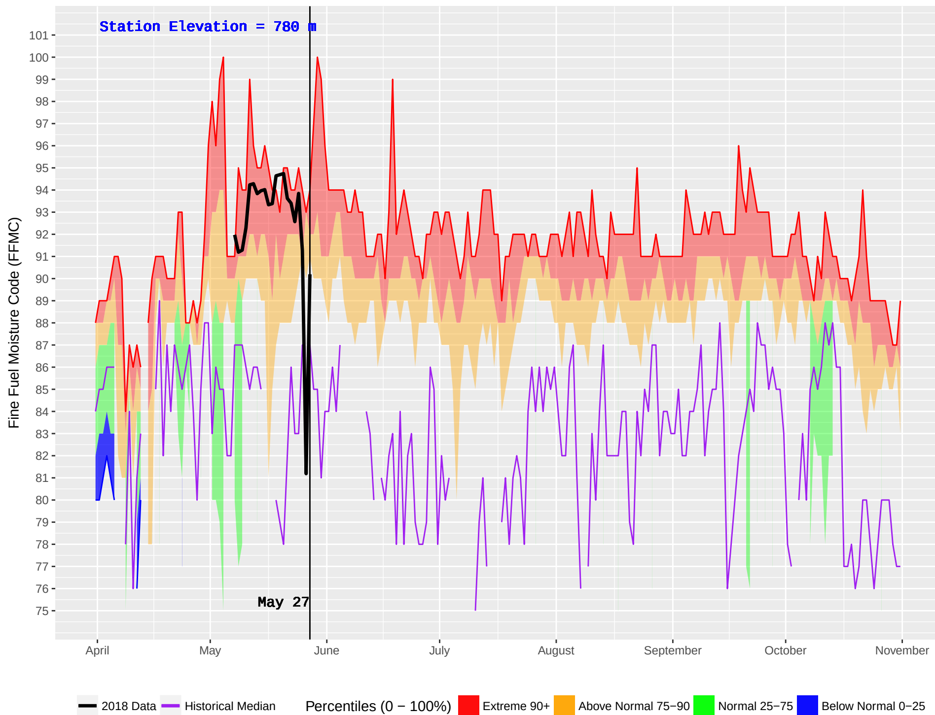
MUSKWA (131) : Historical (1983–2016) and Current (2018) Noon Fine Fuel Moisture Code (FFMC)
